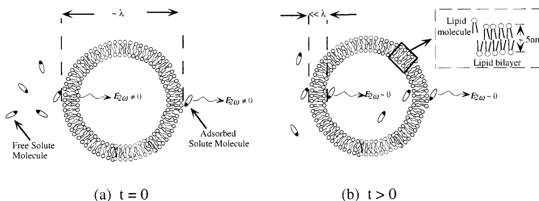
FIGURE 2 Solute molecules are added externally to a liposome suspension. (a) At the early time, the molecules adsorb only to the outer surface of the liposome. Because the size of the liposome is comparable to the wavelength of the light, the second field from the outer surface of the liposome can add coherently and a SHG signal can be observed. (b) When the solute molecules start diffusing into the liposome and adsorb to the inner surface, the second fields, E_{2\omega} , generated at the opposite surface of the bilayer, are separated by the thickness of the bilayer, which is on a length scale much smaller than the wavelength of the light. Therefore they cancel and the second harmonic field, E_{2\omega} , decreases.
