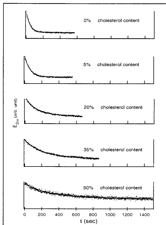
FIGURE 3 The SHG signals decay exponentially with time after a 10 \mu M malachite green (MG) solution is mixed rapidly with the suspensions of liposomes with different cholesterol contents. The total lipid and cholesterol concentration of the samples is kept constant at 12.5 \mu M. The solid lines are the single exponential fit.
